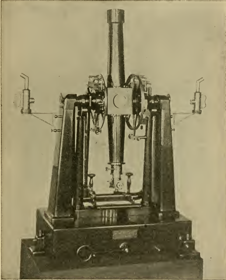
THREE-INCH TRANSIT, BY WARNER & SWASEY.
